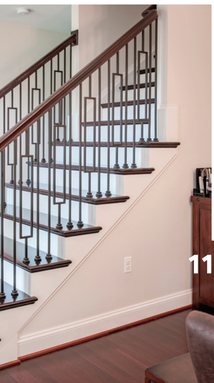
10 LIH-HOL1BASK44, LIH-HOLDBLTW44 Iron Balusters, LJT-3010 Newels, LJ-6010 Handrail and LJ-7031 Climbing Volute
