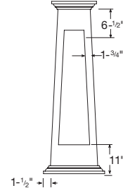
Recess is 1/2" deep and corners are 1/4" rounded.
