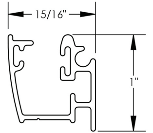
Top Track/ Bottom Track
