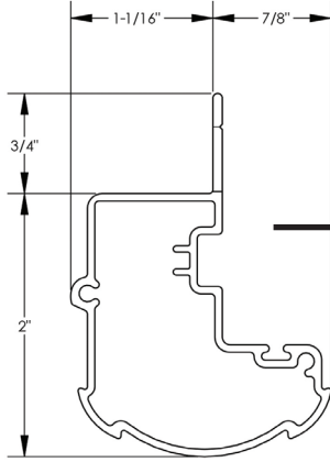
Decorative Housing Profile
