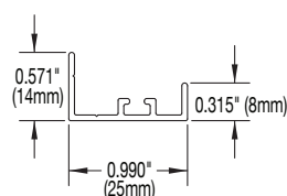
Side Profile
