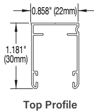
Top Profile
