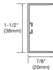
Side Profile
